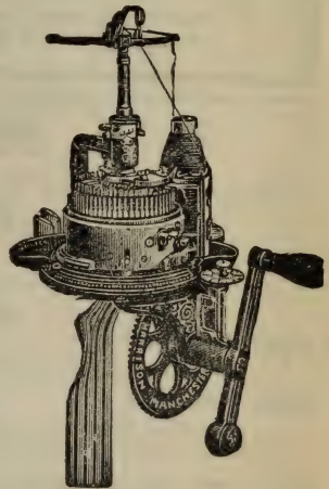
"Harrison" Sun Ribber, for Hose and Half-Hose.
